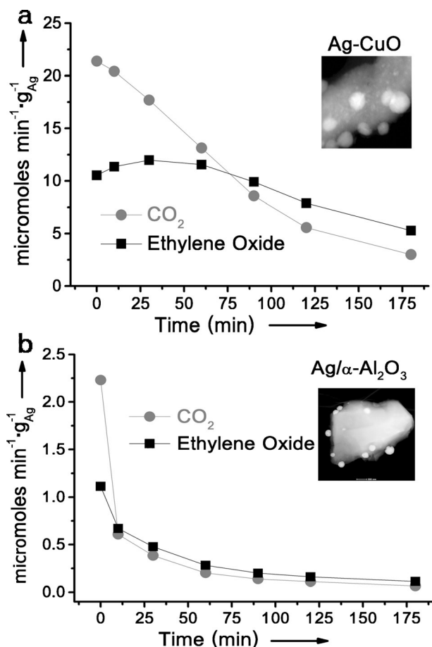
Figure 2. Evolution of the reaction rates of CO 2 and EO during pretreatment with 1,2-dichloroethane (4 ppm) of the a) Ag/CuO catalyst or the b) Ag/Al 2 O 3 catalyst. Temperature = 200 °C. The inlet flow contains 6% ethylene, 12% oxygen, and 88% helium. Insets: STEM-HAADF images of the catalysts (see also the Supporting Information).
