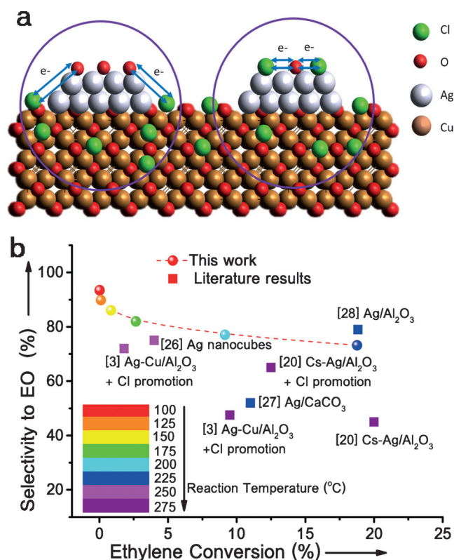
Figure 3. a) Representation of the proposed Cl promotion mechanism; the Cl atoms are readily adsorbed or substituted on both CuO and Ag surfaces and promote the generation of more electrophilic oxygen species in the vicinity; b) Overview of the best reported catalytic performances for ethylene epoxidation expressed in terms of selectivity to EO formation against total ethylene conversion. The Ag/CuO catalyst pretreated with 4 ppm of 1,2-dichloroethane for 180 min (circle symbols) is selected for comparison. Results for previously reported systems are shown as square symbols. The different colors of circles and squares indicate different reaction temperatures (see inset legend). Numbers in square brackets indicate the reference in which the indicated system is reported.
